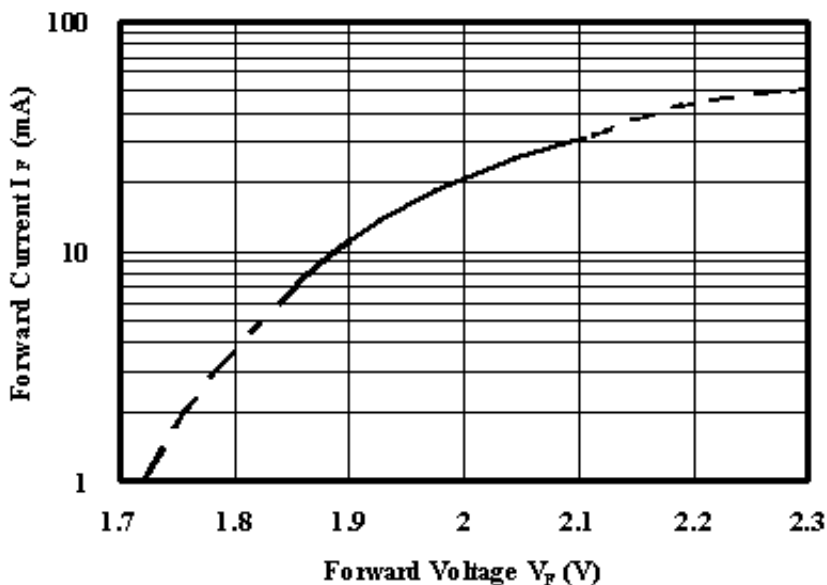
Forward Current vs. Forward Voltage (Ta=25 )
