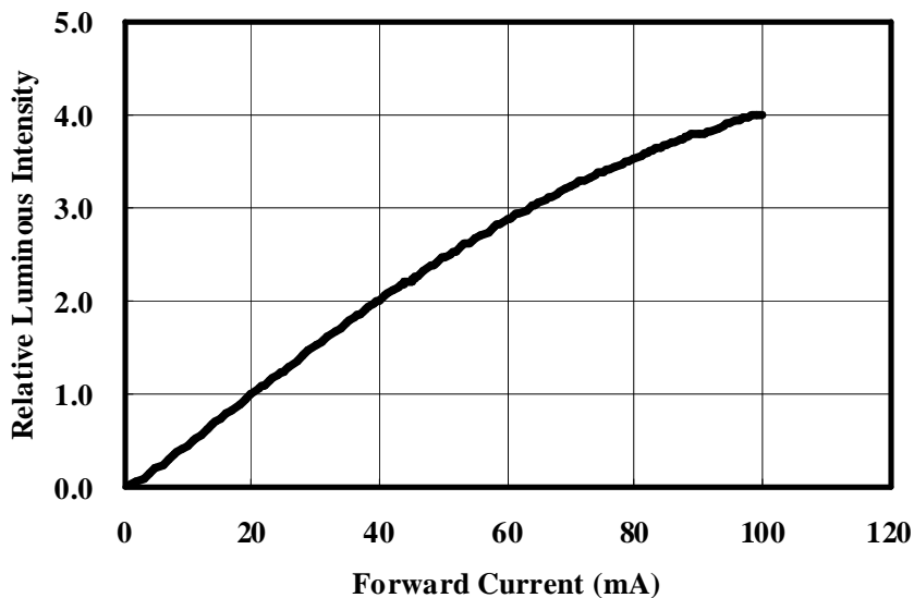
Forward Current vs. Relative Luminous Intensity (Ta=25 )
